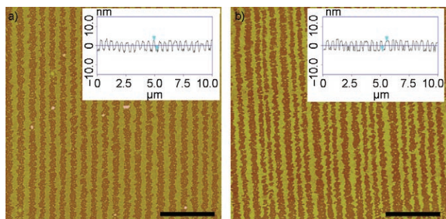
Figure 3. a) AFM image of surface after SIP of styrene with 5 . b) AFM image of surface after SIP of n -butyl acrylate with 5 . (Insets show cross sections; scale bars: 2.5 \mu\text{m} ).
