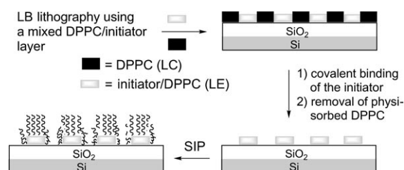
Figure 1. Formation of patterned polymer brushes (LC = liquid condensed phase, LE = liquid expanded phase).
