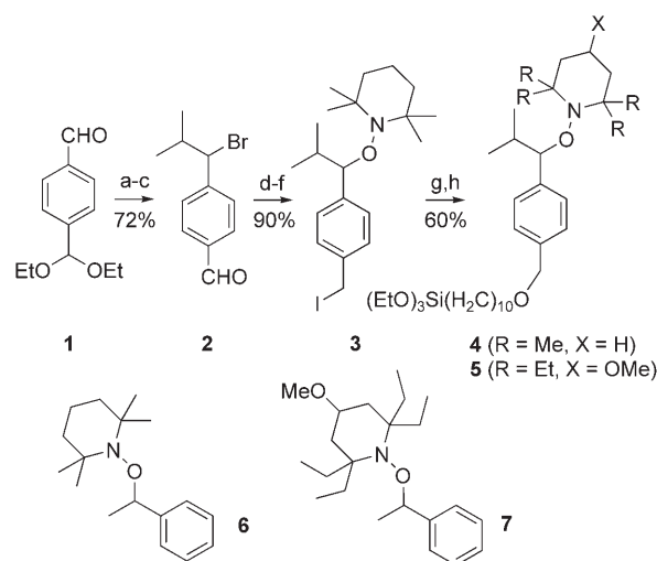
Scheme 1. a) i PrMgCl, Et 2 O; b) aq. HCl; c) HBr (33% in AcOH), CH 2 Cl 2 ; d) TEMPO, Cu, Cu(OTf) 2 (cat.), 4,4'-bis- tert -butylpyridine (cat.), benzene; e) LiAlH 4 , THF; f) TMSCl, NaI, CH 3 CN; g) NaH, CH 2 =CH(CH 2 ) 8 OH, THF; h) HSi(OEt) 3 , Karstedt cat. OTf = trifluoromethanesulfonate; TMS = trimethylsilyl.
