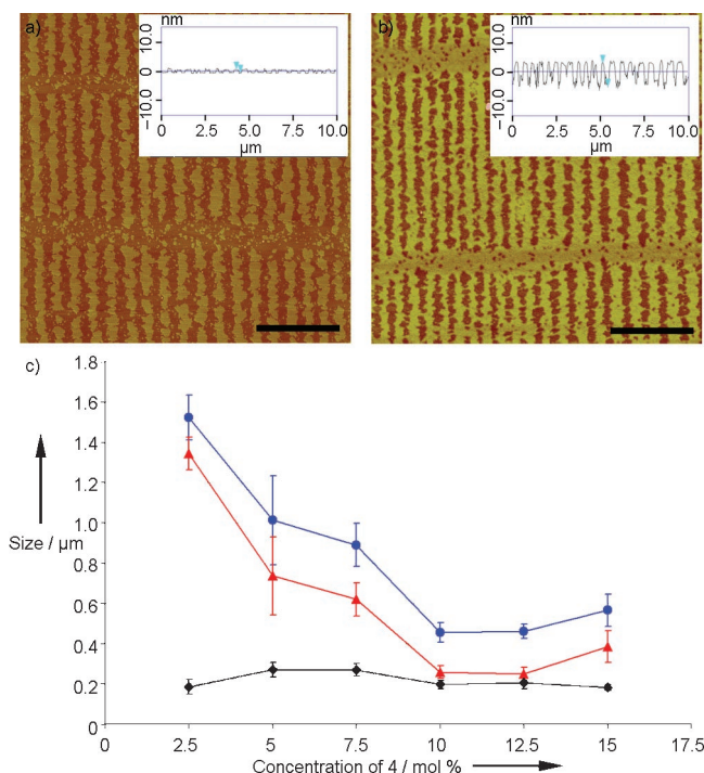
Figure 2. a,b) AFM images of a sample prepared with 10 mol % 4 before (a) and after (b) SIP of styrene (insets show cross sections; scale bars: 2.5 \mu\text{m} ). c) Periodicity (sum of stripe and channel size, blue circles), size of stripes (red triangles), and size of channels (black diamonds) as a function of the concentration of 4 .
